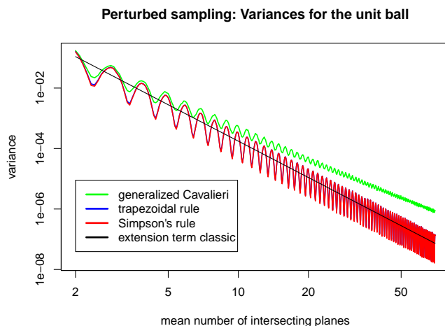
Figure 3: The empirical variance for volume estimation of the unit ball B^3 in \mathbb{R}^3 , shown in a double logarithmic plot. The x -coordinate is 2\gamma and the black line is the extension term (4.1) for the classical Cavalieri estimator with section spacing 1/\gamma .
