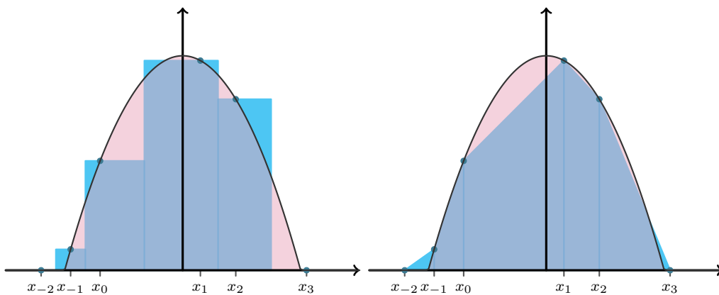
Figure 2: The same measurement function and sample points as in the right of Figure 1, but now the midpoint rule is used (left) leading to non-overlapping rectangles with varying base lengths. The trapezoid rule (right) approximates with a piecewise linear function and leads to the same estimator as the midpoint rule.
