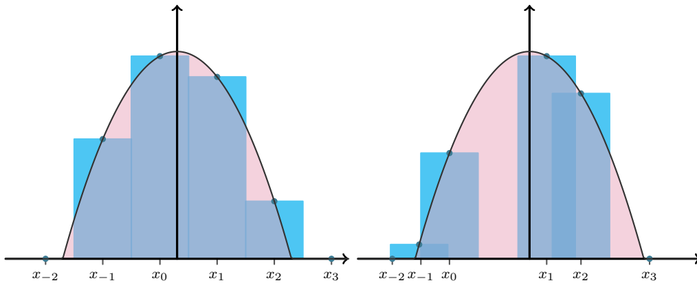
Figure 1: The rectangular quadrature rule for equidistant points ( x_i ) as used in the classical Cavalieri estimator (left) and the corresponding rule when applied to points that are not equidistant (right). The measurement function is in both cases f(x) = 2(1 - x^2) for x \in [-1, 1] .
