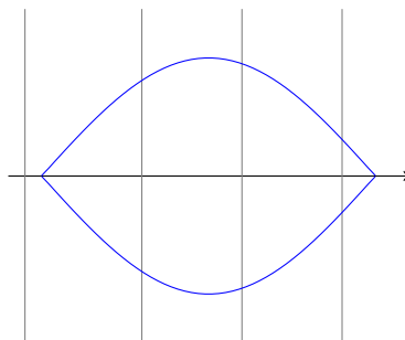
Figure 4: Planar section of a three-dimensional body of revolution through its horizontal rotational axis. The boundary of this spindle is determined by the functions u_{\pm}(x) = \pm\sqrt{(1 + \cos \pi x)/2} , -1 \leq x \leq 1 . The section planes (indicted as vertical lines) are all orthogonal to the rotational axis.
