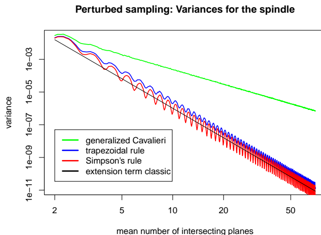
Figure 5: The empirical variances for volume estimation of the spindle S shown in a double logarithmic plot. The x -coordinate is 2\gamma and the black line is the extension term (4.1) for the classical Cavalieri estimator with section spacing 1/\gamma .
