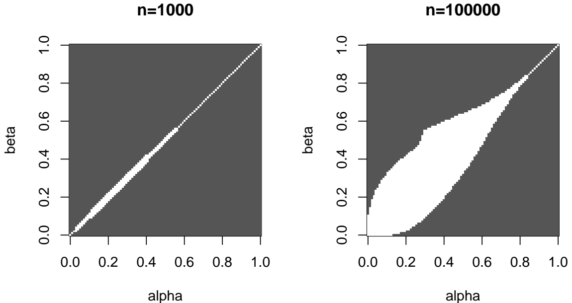
Figure 2: The figure shows the upper bound on the total variation distance from Xia and Zhang (2009) truncated at one. Thus the white region is where the upper bound is below one and the black region is where the bound is above one. The left figure is for n = 1000 and the right figure is for n = 100000 .
