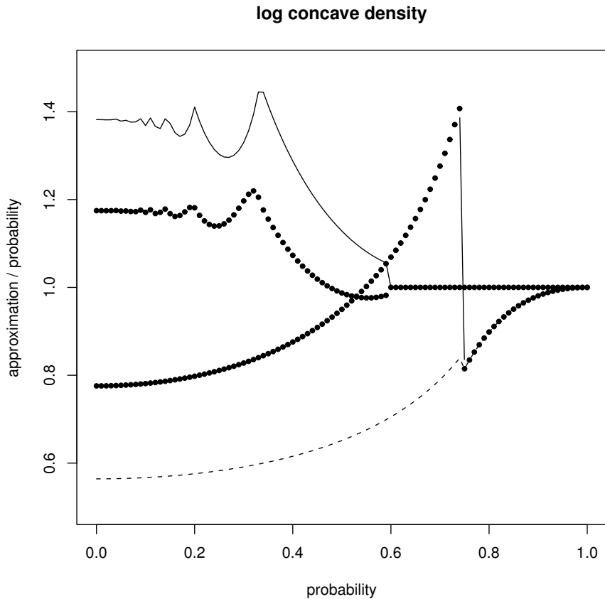
Figure 1: Ratio of saddlepoint approximation to the true probability at the center point for a symmetric log concave density. The full drawn line is for the main term of the saddlepoint approximation and an almost uniform density, and the dashed line is for a discrete Laplace distribution. The dotted lines are for the same cases when using the saddlepoint approximation in (4) and (5).
