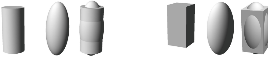
Figure 2: Ellipsoidal approximations to a right circular cylinder and a rectangular parallelepiped in \mathbb{R}^3 .
